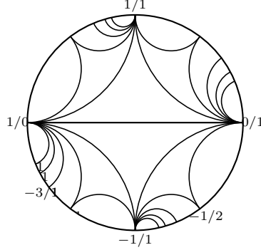
Figure 2: The disk model of the Farey graph
